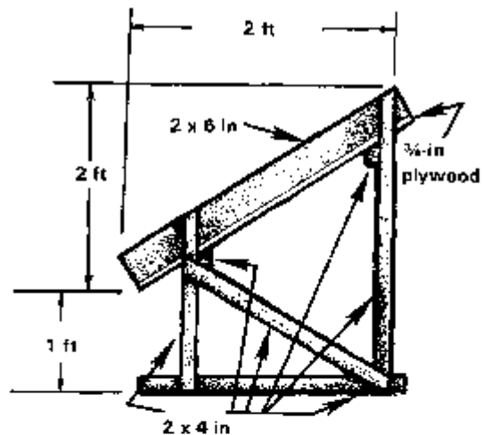
Expedient funnel for filling sandbags
